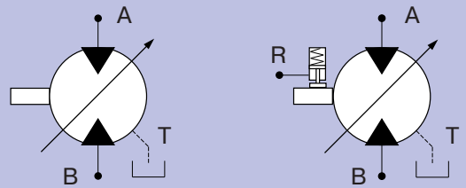
Motor without brake
