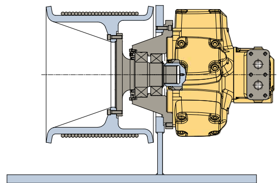
Bracket mounted capstan drive
