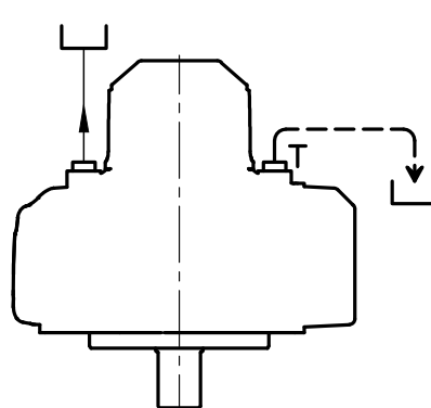
Vertical mounting, shaft downwards, tank located in higher position
